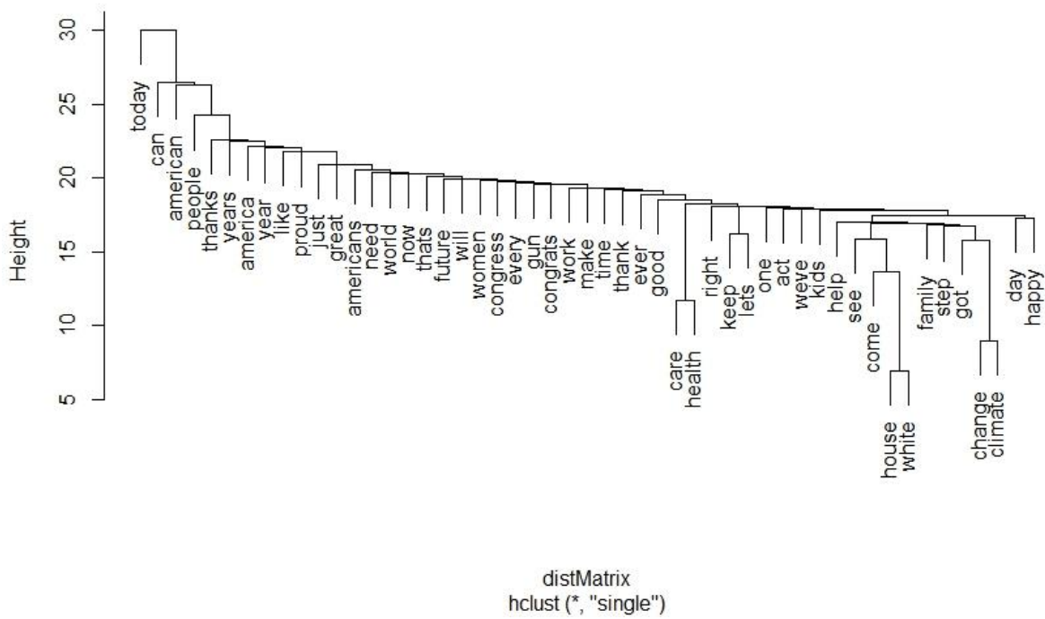
Cluster Dendrogram
