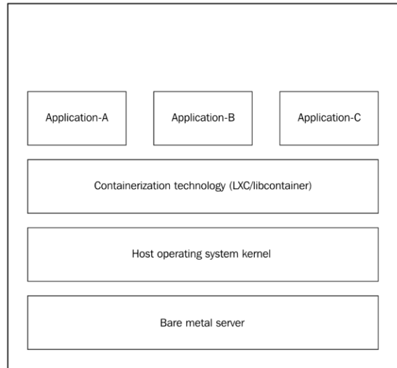
Container
