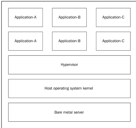
Virtual machine
