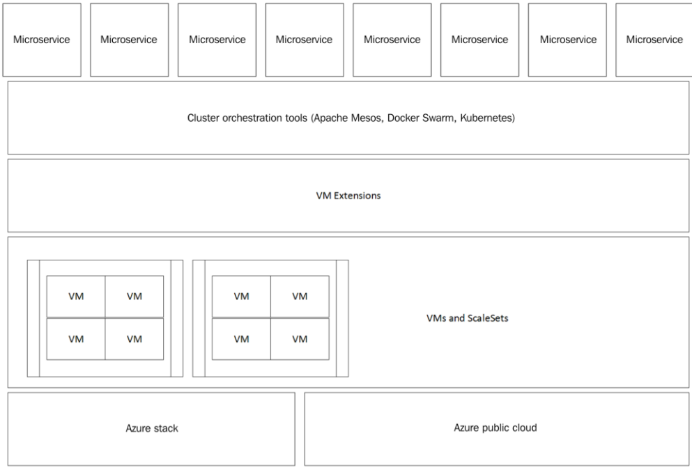
Microservices infrastructure
