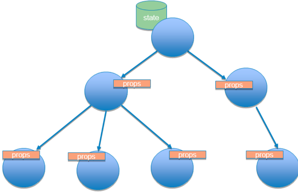
Unidirectional data flow
