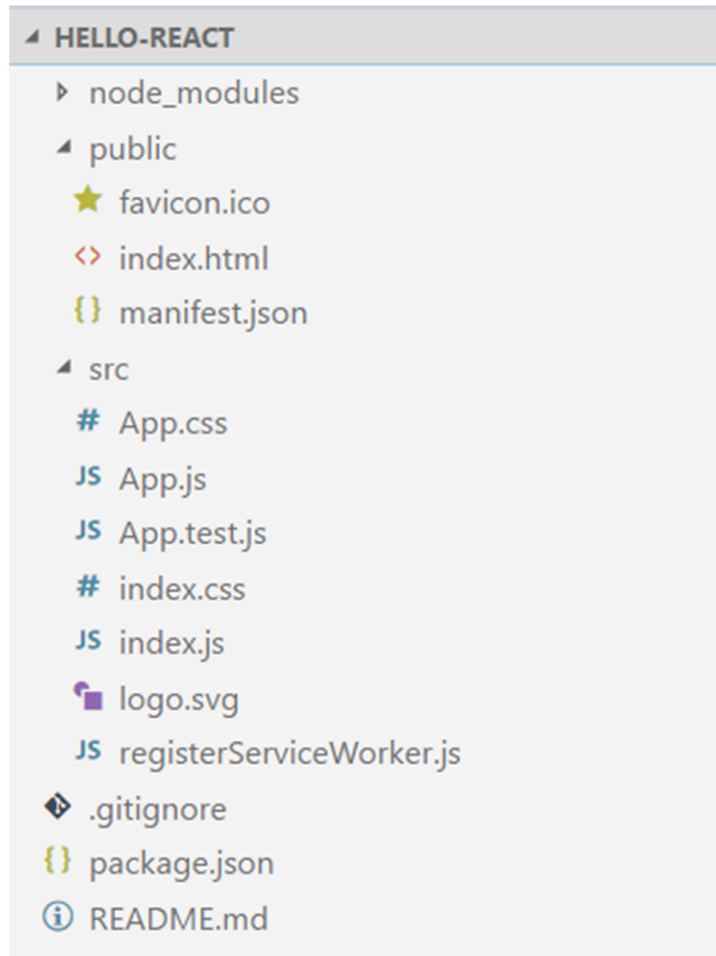
The hello-react folder
