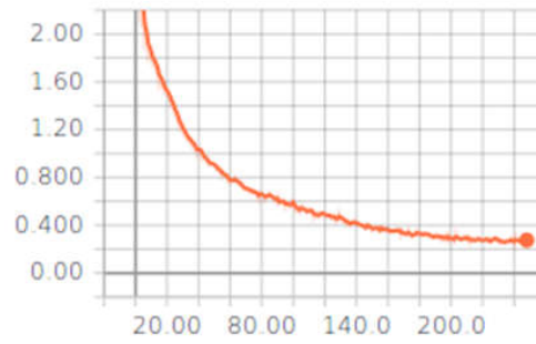
g_loss
