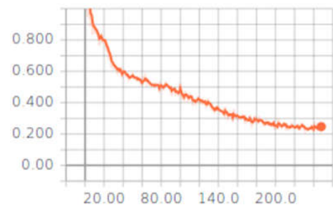
g_loss_b2a
