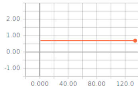
da_loss_fake
