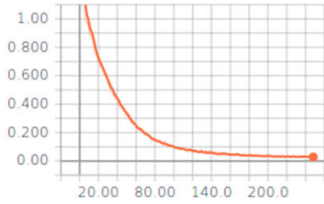
g_loss_a2b
