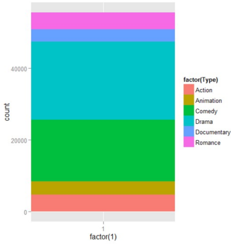
Bar chart with stacked position adjustment
