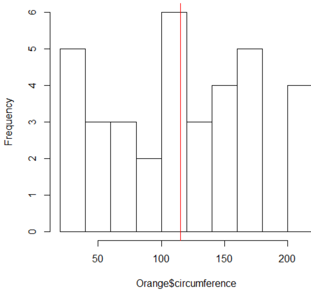
Histogram of Orange$circumference
