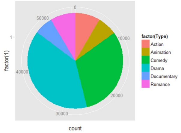
Resulting pie chart with polar coordinates
